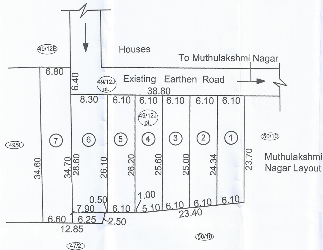
LAYOUT PLAN (Scale-1:50)
